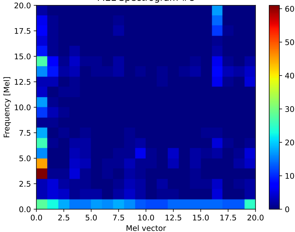
MEL Spectrogram #8
